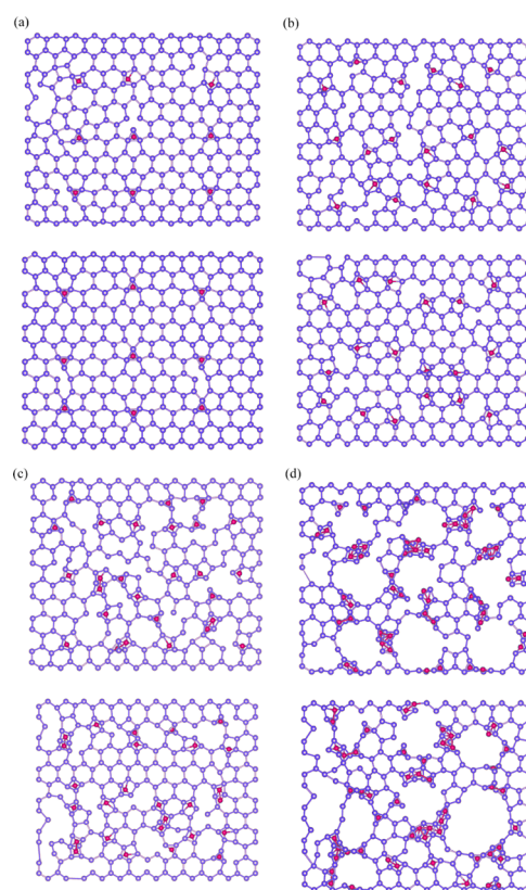
Figure 3. Xy-projections of silicene sheets (upper field—upper sheet, lower field—lower sheet) for various degrees of doping: (a) 3, (b) 6, (c) 9, and (d) 18%.
