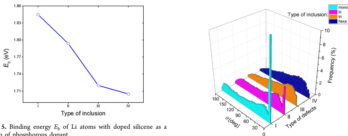
Figure 7. Angular distributions of the nearest geometric neighbors for lithium packings obtained in the final stage of intercalation into the channels of modified silicene with defects (I—mono-, II—bi-, III—tri-, and IV—hexavacancies) originally filled with phosphorus atoms.
