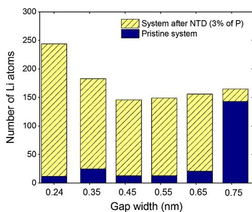
Figure 2. Maximum number of lithium atoms obtained as a result of intercalation in undoped and 3% P-doped silicene channels depending on the gap width h_g between the channel forming sheets.
